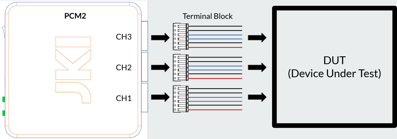
< PCM2 Connection Diagram >
