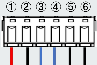
< PCM2 Terminal Assembly >
